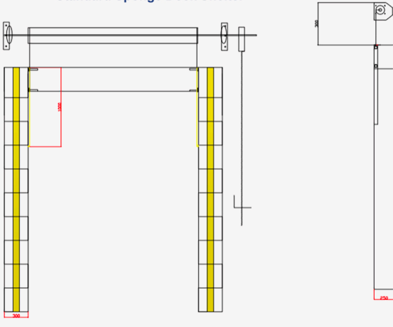
Adjustable Sponge Dock Shelter
